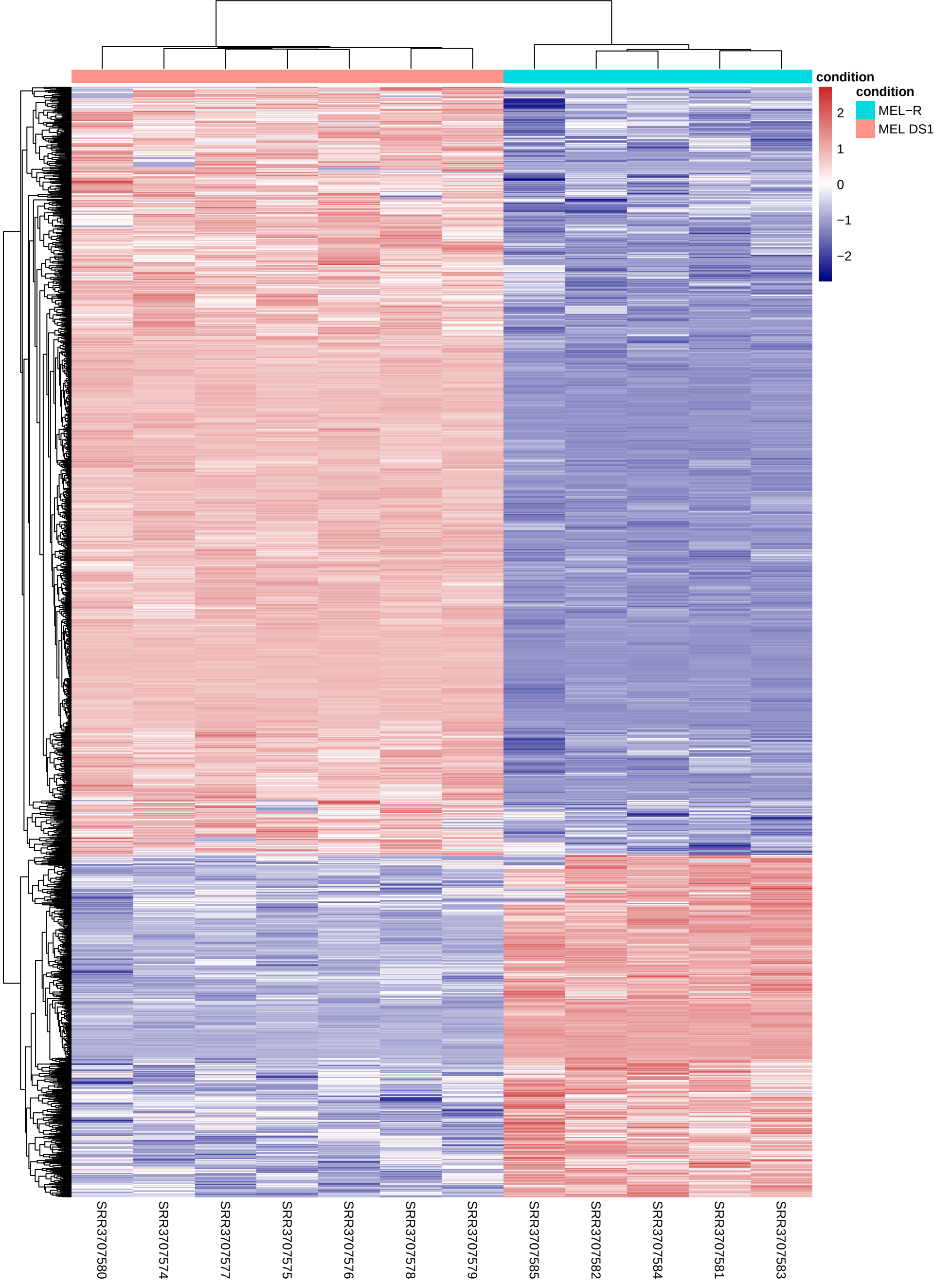
Replication Fig 1A: Global Signature ( |\text{LFC}| > 1 )
